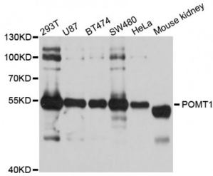
Western blot analysis of extracts of various cell lines, using POMT1 antibody (abx126394) at 1/1000 dilution.
