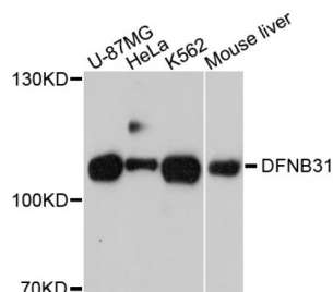
Western blot analysis of extracts of various cell lines, using WHRN antibody (abx126794) at 1/1000 dilution.
