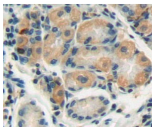
IHC-P analysis of stomach tissue, with DAB staining.
