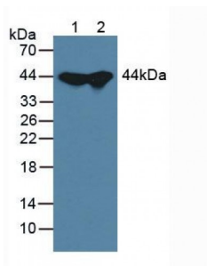
Western blot analysis of (1) Mouse Liver Tissue and (2) Mouse Testis Tissue.
