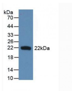
Western blot analysis of recombinant Chicken IFN \beta .
