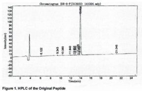
HPLC analysis of unconjugated Human beta Crosslaps Peptide.
