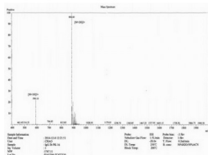
MS analysis of Immunoglobulin G2b Protein (OVA).
