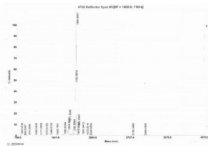
MS analysis of N-Telopeptide Of Type I Collagen Protein (OVA).
