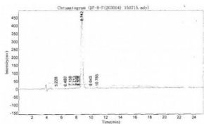
HPLC analysis of Amyloid beta Peptide 1-40 (OVA).
