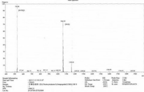
MS analysis of Cholecystokinin 8, Octapeptide (BSA).
