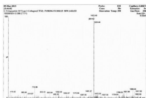
Mass spectrometry analysis of Human CTXI (prior to conjugation).
