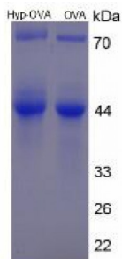
SDS-PAGE analysis of Hydroxyproline (OVA).
