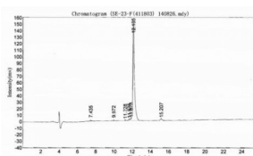
HPLC analysis of Urocortin 1 Protein (OVA).
