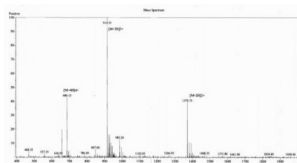
MS analysis of Urocortin 1 Protein (OVA).
