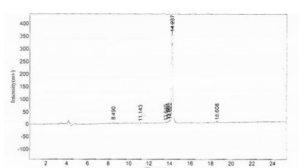
HPLC analysis of Von Willebrand Factor Protein (OVA).
