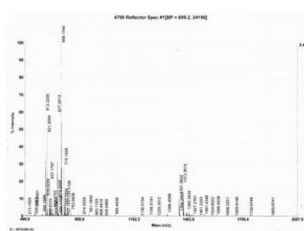
MS analysis of Enkephalin Protein (OVA).
