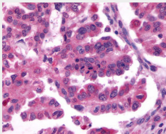
Anti-CXCR4 antibody IHC of human Ovary, Carcinoma.
