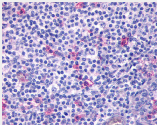
Anti-CXCR4 antibody ALS10342 IHC of human tonsil.
