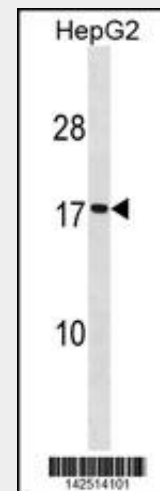
SEC11A Antibody (Center) (Cat. #AP20099c) western blot analysis in HepG2 cell line lysates (35ug/lane). This demonstrates the SEC11A antibody detected the SEC11A protein (arrow).
