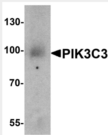
Western blot analysis of PIK3C3 in mouse small intestine tissue lysate with PIK3C3 antibody at 1 µg/ml.
