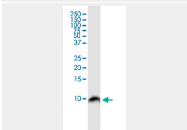
BANF1 monoclonal antibody (M07), clone M2. Western Blot analysis of BANF1 expression in Raw 264.7.
