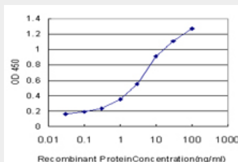
Detection limit for recombinant GST tagged FH is approximately 0.1ng/ml as a capture antibody.
