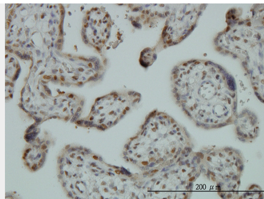
Immunoperoxidase of monoclonal antibody to FUBP1 on formalin-fixed paraffin-embedded human placenta. [antibody concentration 3 ug/ml]
