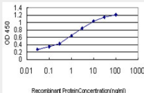
Detection limit for recombinant GST tagged FUBP1 is approximately 0.03ng/ml as a capture antibody.
