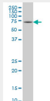
HSPA2 monoclonal antibody (M02), clone 3H7 Western Blot analysis of HSPA2 expression in HepG2 ( Cat # AT2447a )
