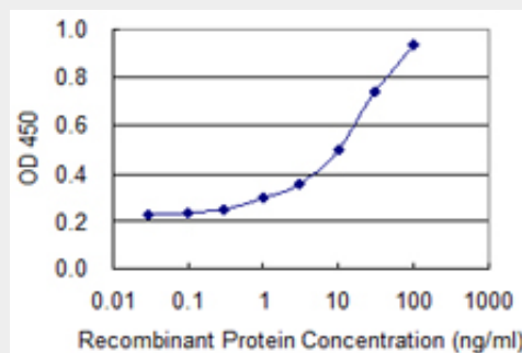
Detection limit for recombinant GST tagged HSPA2 is 0.3 ng/ml as a capture antibody.
