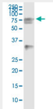
Immunoprecipitation of HSPA2 transfected lysate using anti-HSPA2 monoclonal antibody and Protein A Magnetic Bead ( U0007 ), and immunoblotted with HSPA2 MaxPab rabbit polyclonal antibody.
