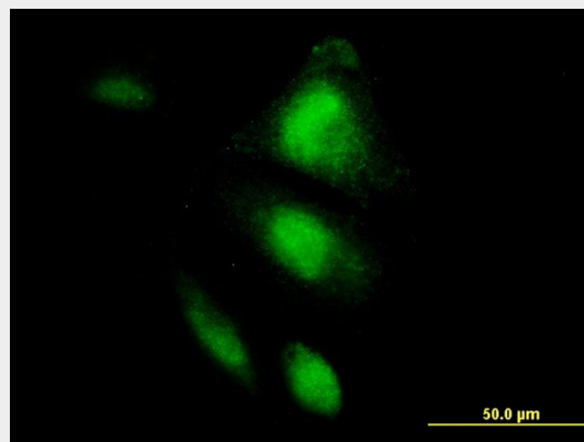
Immunofluorescence of monoclonal antibody to HSPA2 on HepG2 cell. [antibody concentration 10 ug/ml]
