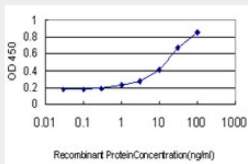
Detection limit for recombinant GST tagged MMP26 is approximately 1ng/ml as a capture antibody.
