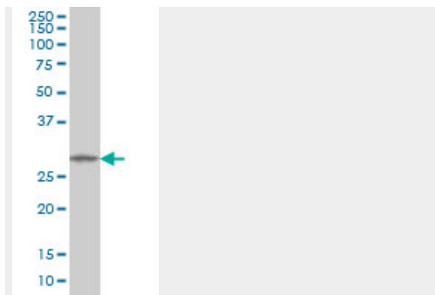
MMP26 monoclonal antibody (M01), clone 6C6 Western Blot analysis of MMP26 expression in HL-60 (Cat # AT2881a)
