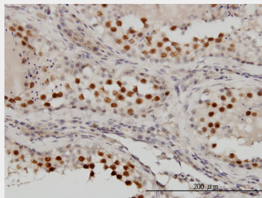
Immunoperoxidase of monoclonal antibody to RACGAP1 on formalin-fixed paraffin-embedded human testis. [antibody concentration 1 ug/ml]
