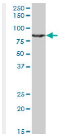
RACGAP1 monoclonal antibody (M01), clone 1G6. Western Blot analysis of RACGAP1 expression in Jurkat (Cat # AT3542a)
