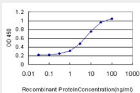
Detection limit for recombinant GST tagged RACGAP1 is approximately 0.3ng/ml as a capture antibody.
