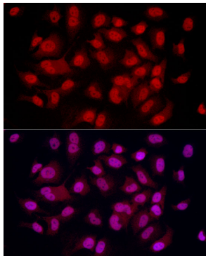
Immunofluorescence analysis of HeLa cells using TriMethyl-Histone H3-K4 Rabbit mAb (A22226) at dilution of 1:100(40x lens). Secondary antibody: Cy3-conjugated Goat anti-Rabbit IgG (H+L) (AS007) at 1:500 dilution. Blue: DAPI for nuclear staining.
