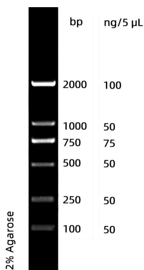
DL2000 plus DNA Marker
