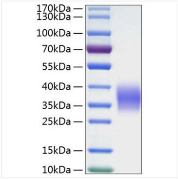
Active Recombinant Human Ephrin-B2/EFNB2 Protein was determined by SDS-PAGE with Coomassie Blue, showing a band at 30-40 kDa.
