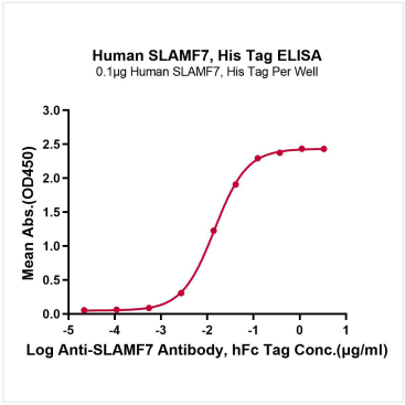
Immobilized Human SLAMF7, His Tag at 1 µg/mL (100 µL/well) on the plate. Dose response curve for Anti-SLAMF7 Antibody, hFc Tag with the EC 50 of 14.3ng/mL determined by ELISA.
