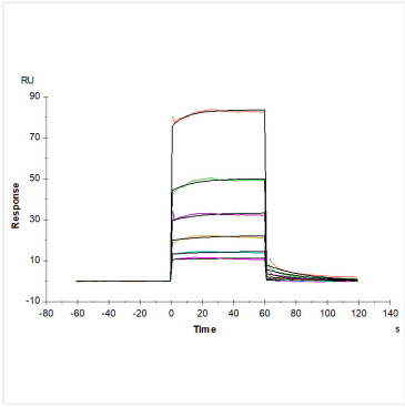
Human TREM2, hFc Tag captured on CM5 Chip via Protein A can bind Human APOE3, His Tag with an affinity constant of 1.21 μM as determined in SPR assay (Biacore T200).
