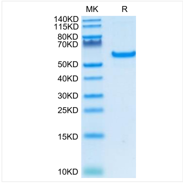
Human CD40 on Tris-Bis PAGE under reduced condition. The purity is greater than 95%.
