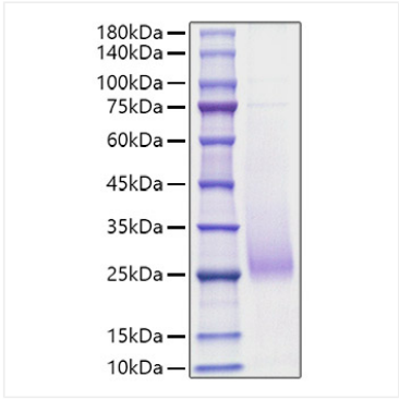
Recombinant Human CD70/TNFSF7/CD27 Ligand Protein was determined by SDS-PAGE with Coomassie Blue, showing a band at 22 kDa.
