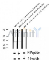
Western blot analysis of extracts of MKN-45 cells treated with Forskolin, using Phospho-DARPP-32 (Ser97) Ab.
