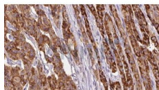
AF2365 at 1/100 staining Human thyroid cancer tissue by IHC-P. The sample was formaldehyde fixed and a heat mediated antigen retrieval step in citrate buffer was performed. The sample was then blocked and incubated with the Ab for 1.5 hours at 22°C. An HRP conjugated goat anti-rabbit Ab was used as the secondary.
