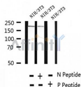
Western blot analysis of extracts of NIH/3T3 cells, using Phospho-Tuberin/TSC2 (Ser939) Ab.
