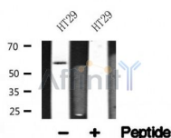
Western blot analysis of PHGDH in lysates of HT29, using PHGDH Ab(AF4618).
