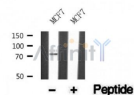
Western blot analysis of Gab2 in lysates of MCF7, using Gab2 Ab(AF4803).
