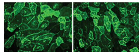
HUVECs with Tagged GFP on Cell Membrane for Permeability Studies
