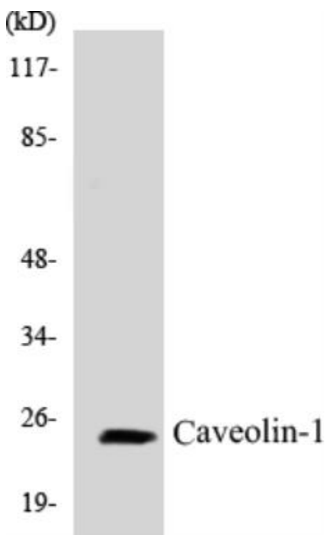
Figure 2. Western blot analysis of extracts from NIH-3T3 cells, using Caveolin-1 (Ab-14) Antibody.
