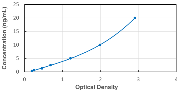
Typical Standard Curve for Mouse IGFBP2 ELISA
