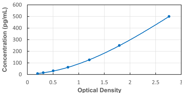
Typical Standard Curve for Human IL8 ELISA
