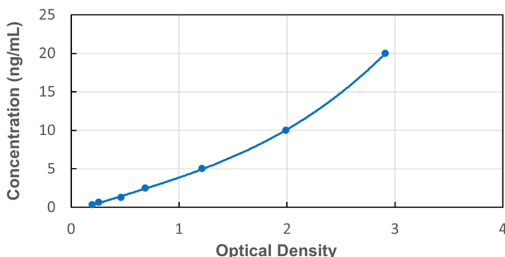
Typical Standard Curve for Human APOM ELISA
