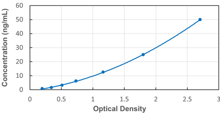
Typical Standard Curve for Human CLU ELISA
