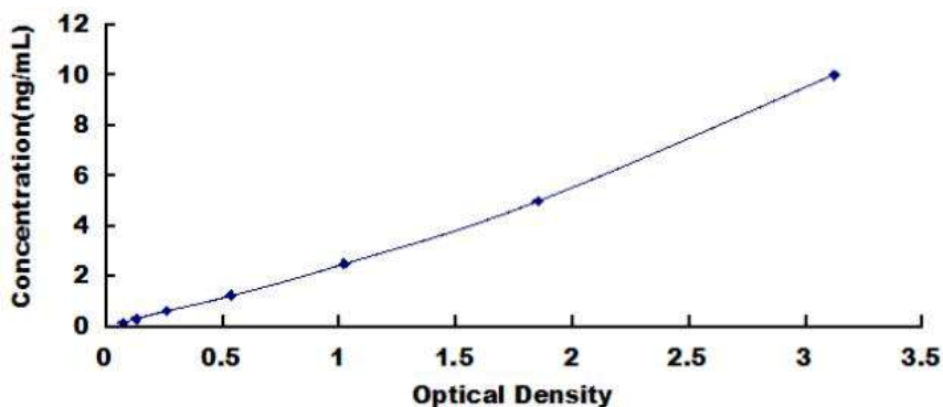
Typical Standard Curve for Human HNRPA2B1 ELISA.
