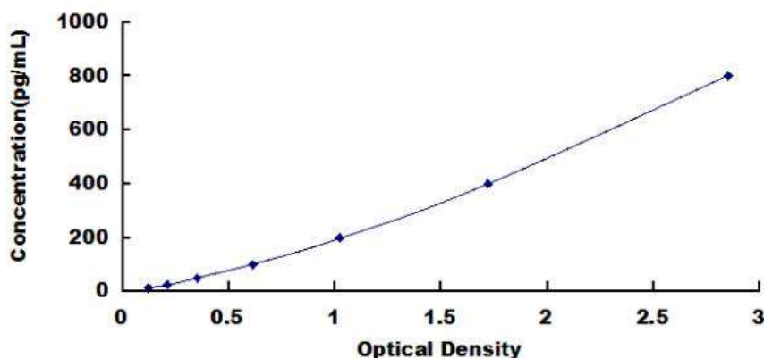
Typical Standard Curve for Mouse LOX1 ELISA.
