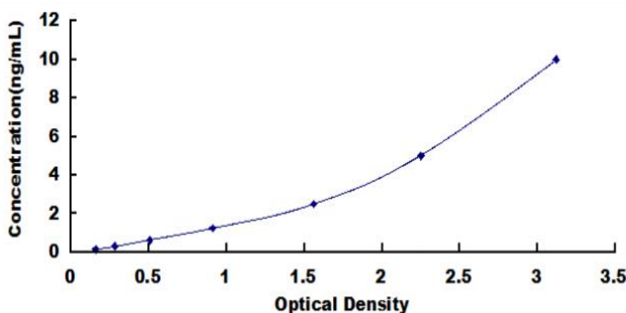
Typical Standard Curve for SLURP1 ELISA.
