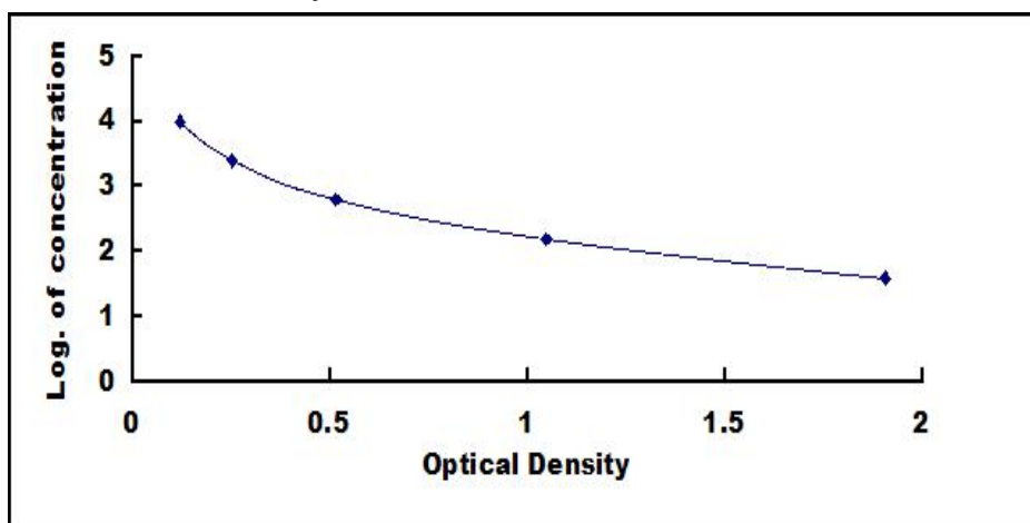
Typical Standard Curve for KS ELISA.
