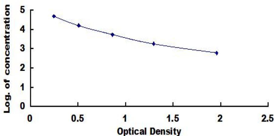
Typical Standard Curve for sIgA ELISA.
