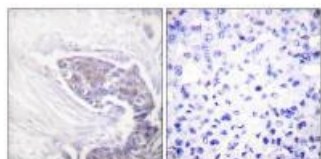
Immunohistochemistry analysis of paraffin-embedded human breast carcinoma tissue using TRXR2 antibody A03900.
