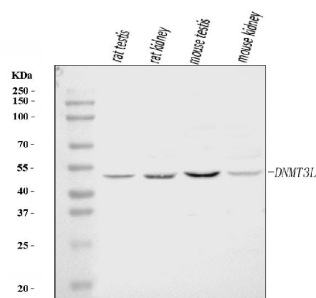
Figure 1. Western blot analysis of DNMT3L using anti-DNMT3L antibody (A04214-3). Electrophoresis was performed on a 5-20% SDS-PAGE gel at 70V (Stacking gel) / 90V (Resolving gel) for 2-3 hours. The sample well of each lane was loaded with 30 ug of sample under reducing conditions.
