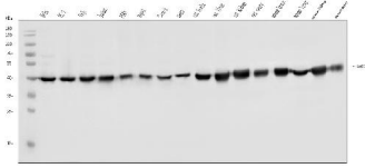
Figure 1. Western blot analysis of FABP-1/GOT2 using anti-FABP-1/GOT2 antibody (A05998-1). Electrophoresis was performed on a 5-20% SDS-PAGE gel at 70V (Stacking gel) / 90V (Resolving gel) for 2-3 hours. The sample well of each lane was loaded with 30ug of sample under reducing conditions.
