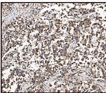
Figure 10. IHC analysis of FABP-1/GOT2 using anti-FABP-1/GOT2 antibody (A05998-1). FABP-1/GOT2 was detected in paraffin-embedded section of human gastric cancer tissue. Heat mediated antigen retrieval was performed in EDTA buffer (pH8.0, epitope retrieval solution). The tissue section was blocked with 10% goat serum. The tissue section was then incubated with 2ug/ml rabbit anti-FABP-1/GOT2 Antibody (A05998-1) overnight at 4°C. Biotinylated goat anti-rabbit IgG was used as secondary antibody and incubated for 30 minutes at 37°C. The tissue section was developed using Streptavidin-Biotin-Complex (SABC) (Catalog # SA1022) with DAB as the chromogen.
