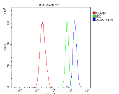
Figure 2. Flow Cytometry analysis of U20S cells using anti-Annexin VIII antibody (A08645).
